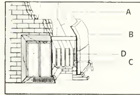
Shown at left, foil insulation A, fiberglass insulation B, water inlet C, and part of the 40 sq. ft. water pipe surface D that, with a 1,000 gal. heat storage tank, warms room air for up to 48 hrs.
